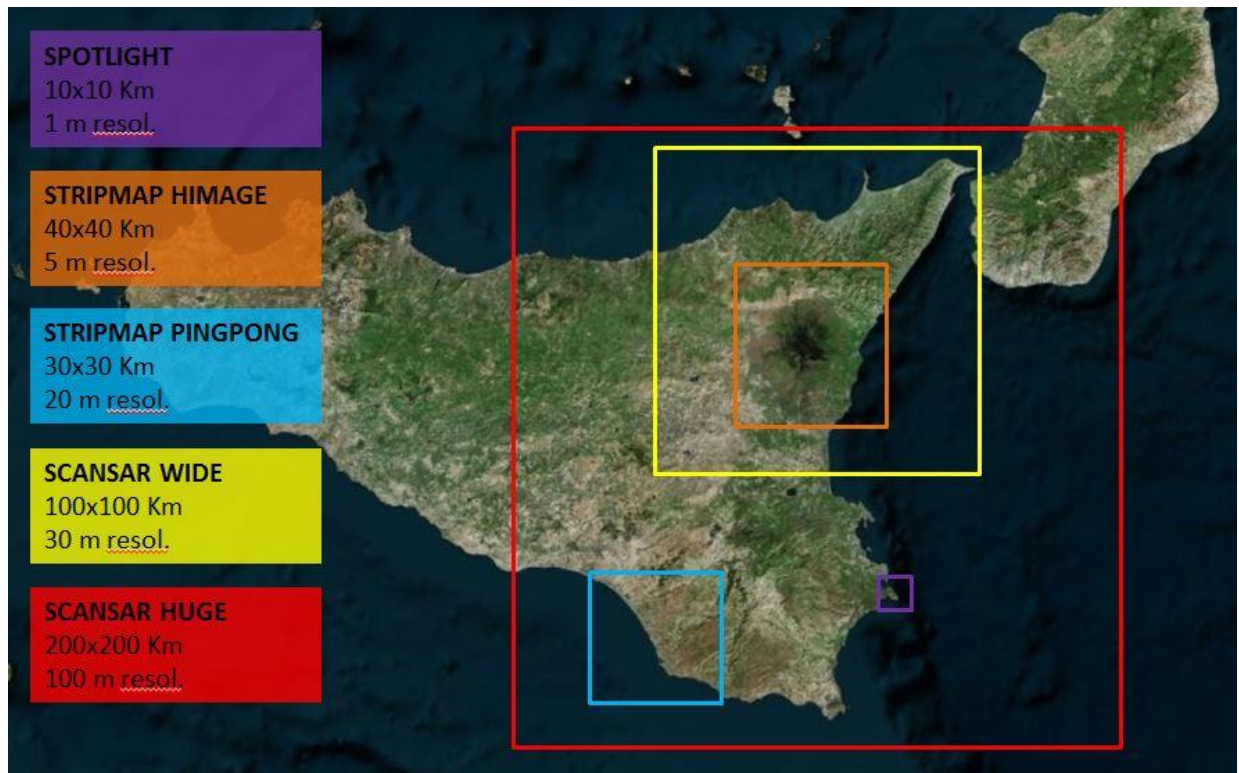
Figure 12 – A pictorial view of the 5 major types of COSMO-SkyMed Acquisition Modes
