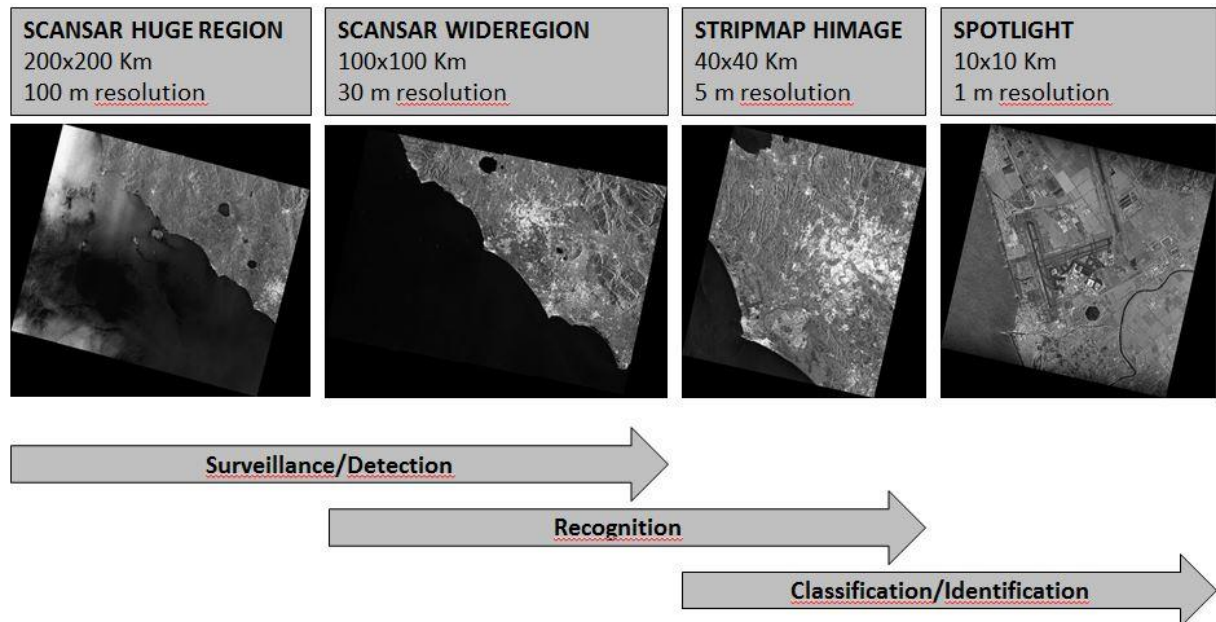
Figure 1 – The acquisition modes of COSMO-SkyMed sensor
